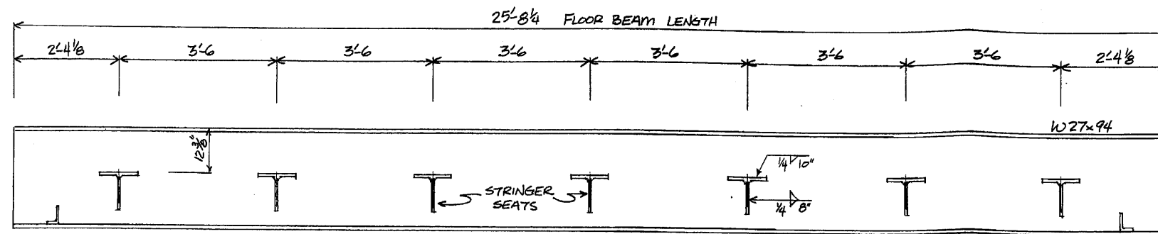
FLOOR BEAM DETAIL
