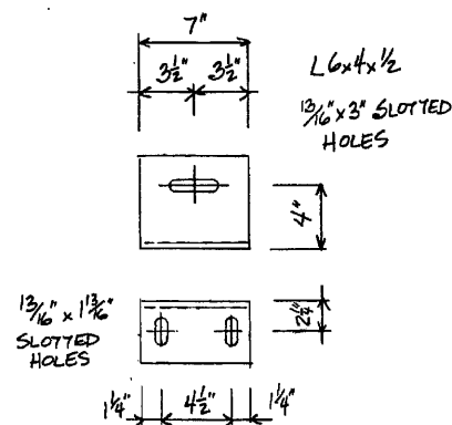
ANGLE A 36 REQ'D
