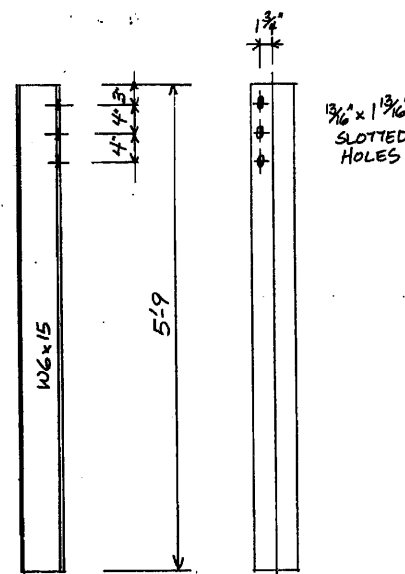
POST A - 4 REQ'D
