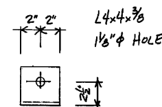
ANGLE C 4 REQ'D
