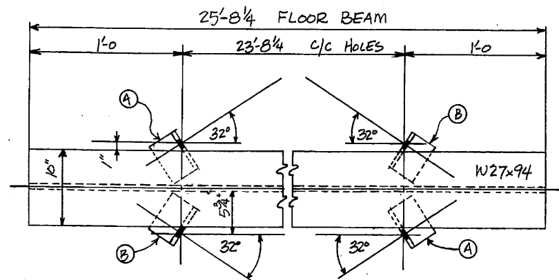
LATERAL ROD ANCHOR LAYOUT
