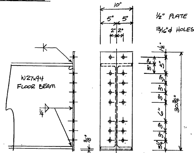
FLOOR BEAM DETAIL
