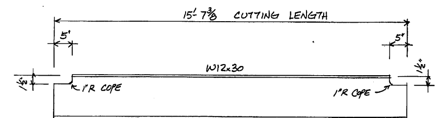
INTERIOR PANEL STRINGERS 49 REQ'D
