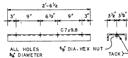
SPLICE CHANNEL 8 REQUIRED
