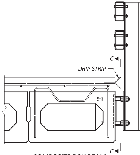
COMPOSITE BOX BEAM WITH TST-1-99 RAILING (DECK ON CONCRETE OR STEEL BEAM SIMILAR)
