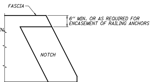
PLAN-FASCIA BEAM WITH NOTCH
