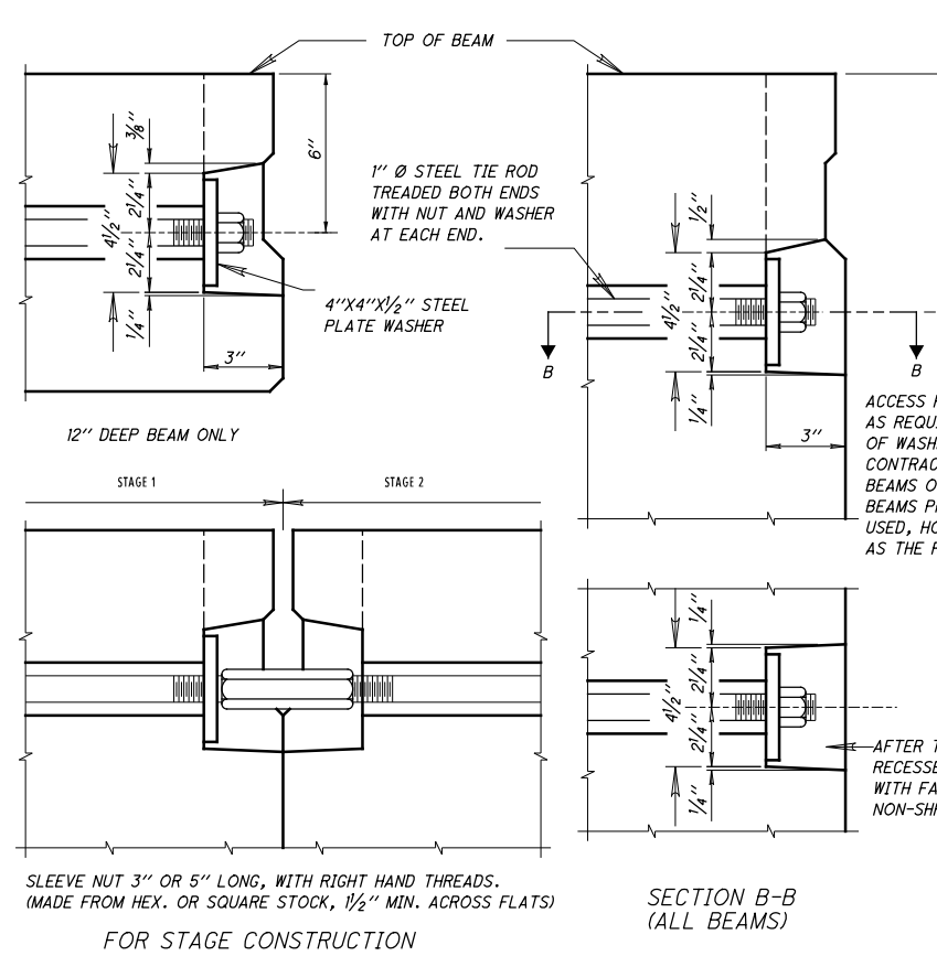
END DETAILS OF TRANSVERSE TIE ROD ANCHORAGE
