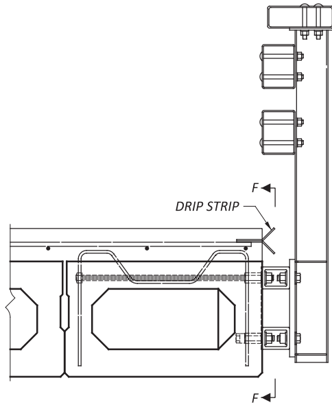
COMPOSITE BOX BEAM WITH TST-2-21 RAILING (DECK ON CONCRETE OR STEEL BEAM SIMILAR)
