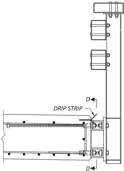
CONCRETE SLAB WITH TST-2-21 RAILING (DECK ON CONCRETE OR STEEL BEAM SIMILAR)
