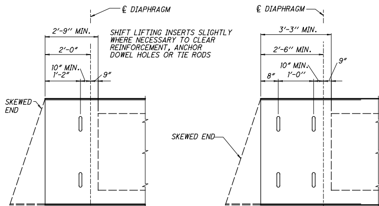
FOR 12", 17" AND 21" DEEP BEAMS
