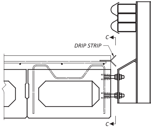
COMPOSITE BOX BEAM WITH DBR-2-73 RAILING (DECK ON CONCRETE OR STEEL BEAM SIMILAR)
