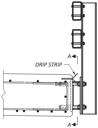
CONCRETE SLAB WITH TST-1-99 RAILING (DECK ON CONCRETE OR STEEL BEAM SIMILAR)
