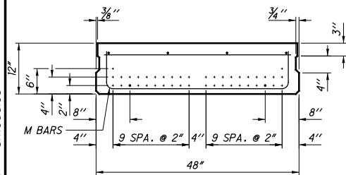
B12-48 (STRAND PATTERN TYPICAL FOR ALL 48" WIDE BEAMS)
